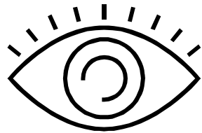
BIOMETRICS / MICRO-EXPRESSIONS
