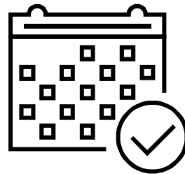
CREDIT SCORING
